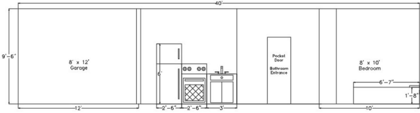
8' x 40' Container 6 Front Internal Elevation 4/16/2025
