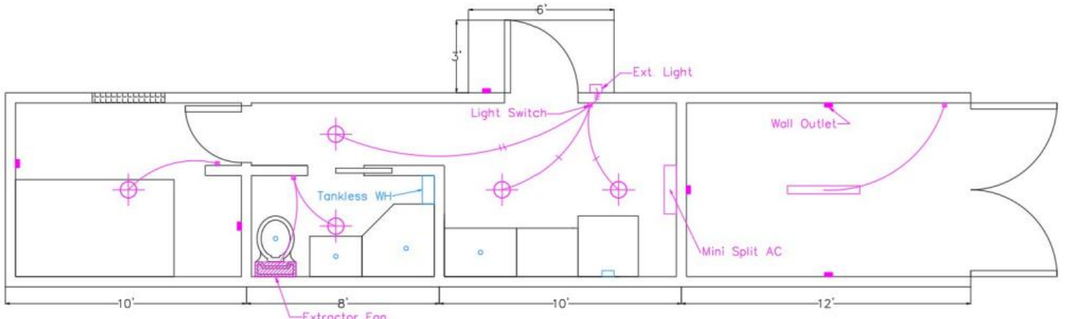
8' x 40' Container 6 Electric and Water Plan
