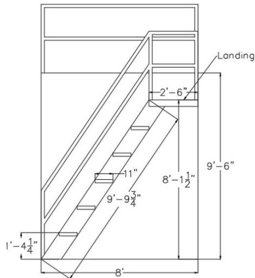
8' x 40' Container 6 Side External View
