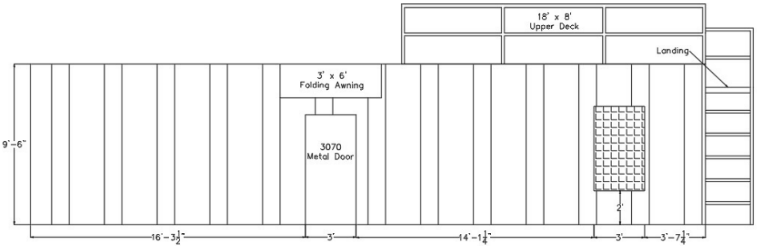
8' x 40' Container 6 Front External Elevation
