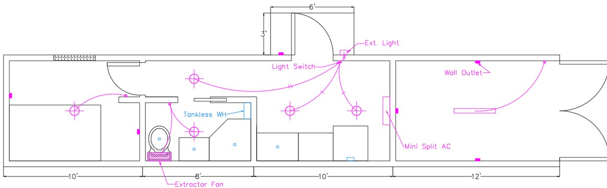
8' x 40' Container 6 Electric and Water Plan 4/16/2025
