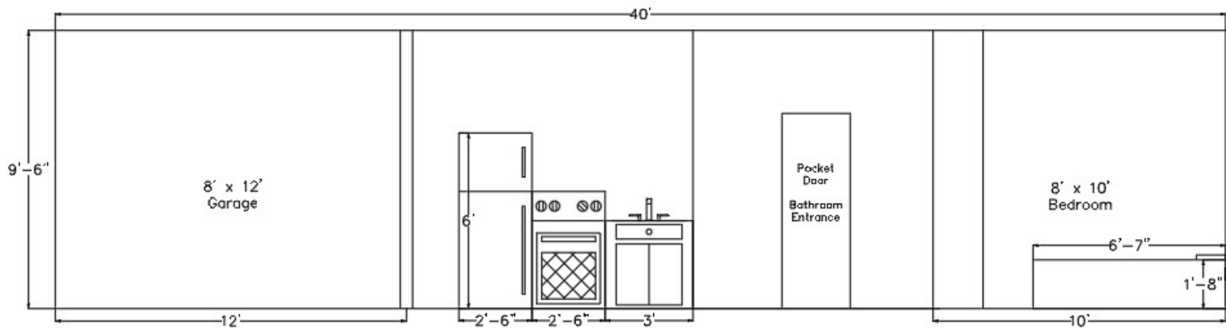
8' x 40' Container 6 Front Internal Elevation 4/16/2025
