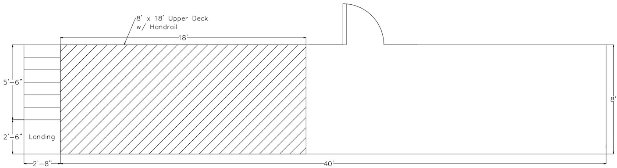
8' x 40' Container 6 Upper Deck View
