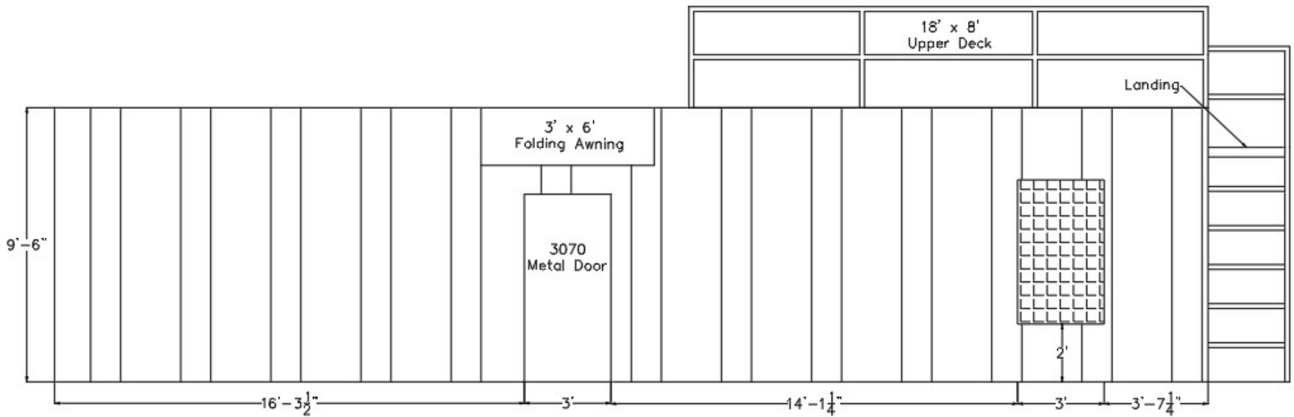
8' x 40' Container 6 Front External Elevation 4/16/2025
