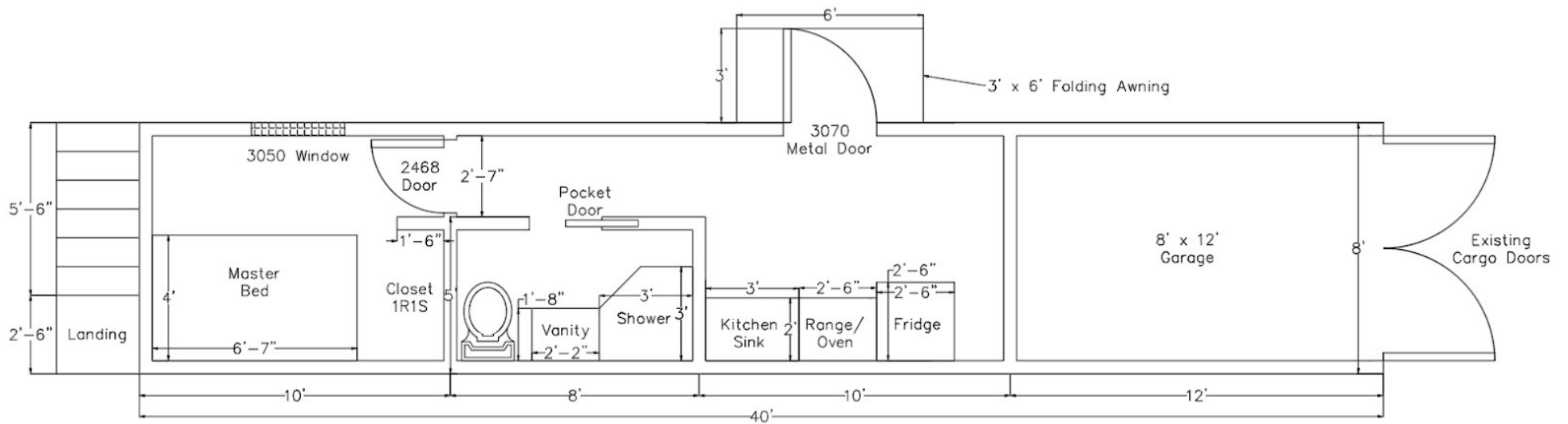
8' x 40' Container 6 Floor Plan 4/16/2025
