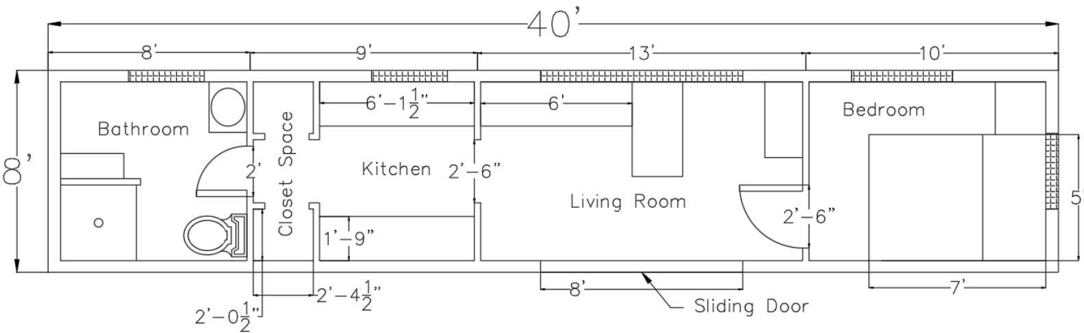
8' x 40' Shipping Container Floor Plan 06/10/2024
