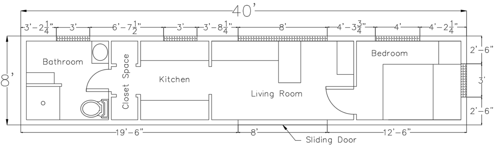
8' x 40' Shipping Container Opening Plan 06/10/2024
